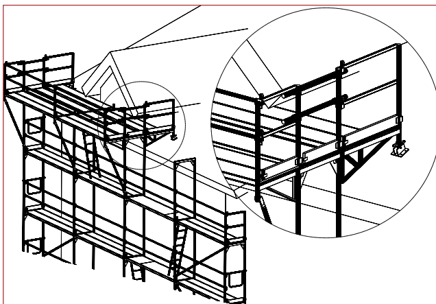
fig. 8.4 – Attic set-up 1
