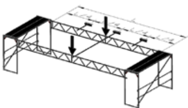
Upper belt stabilisation
